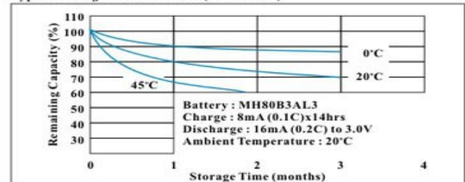
Typical Storage Characteristics (Button Cell)
