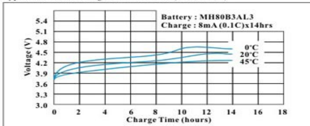
Typical Quick Charge Characteristics (Button Cell)
