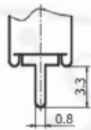
PC-V terminal (4)
