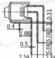
PC-V terminal (4)
