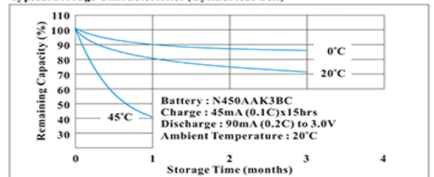
Typical Storage Characteristics (Cylindrical Cell)
