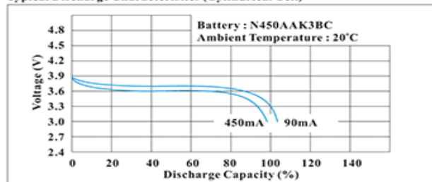
Typical Discharge Characteristics (Cylindrical Cell)
