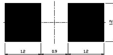
Recommended Soldering Pad Dimensions
