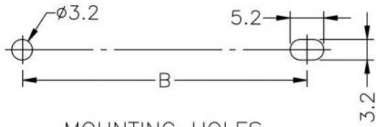
MOUNTING HOLES CHASSIS THICKNESS:0.8~1.2
