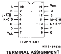
92CS-24835 TERMINAL ASSIGNMENT
