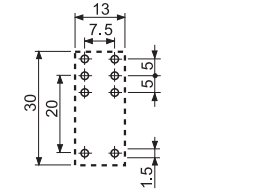
95.15.2 Copper side view
