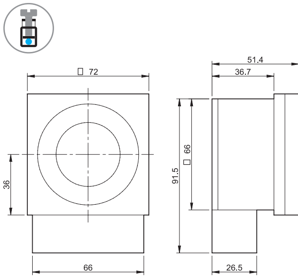
12.71 Screw terminal
