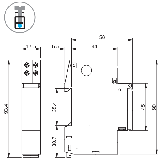
12.11 Screw terminal
