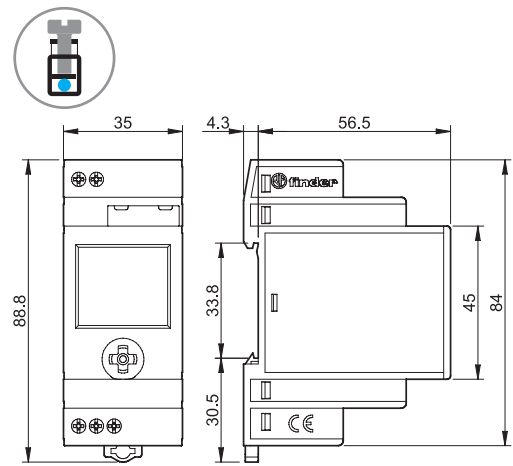
12.51/12.81 Screw terminal
